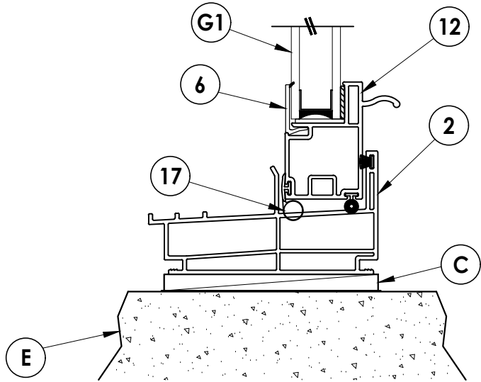
2 3 VERTICAL CROSS SECTION Shown direct to masonry
