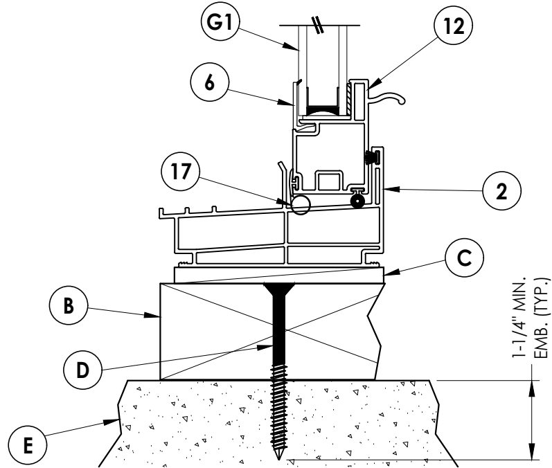
2 3 VERTICAL CROSS SECTION Shown w/ 2X buck
